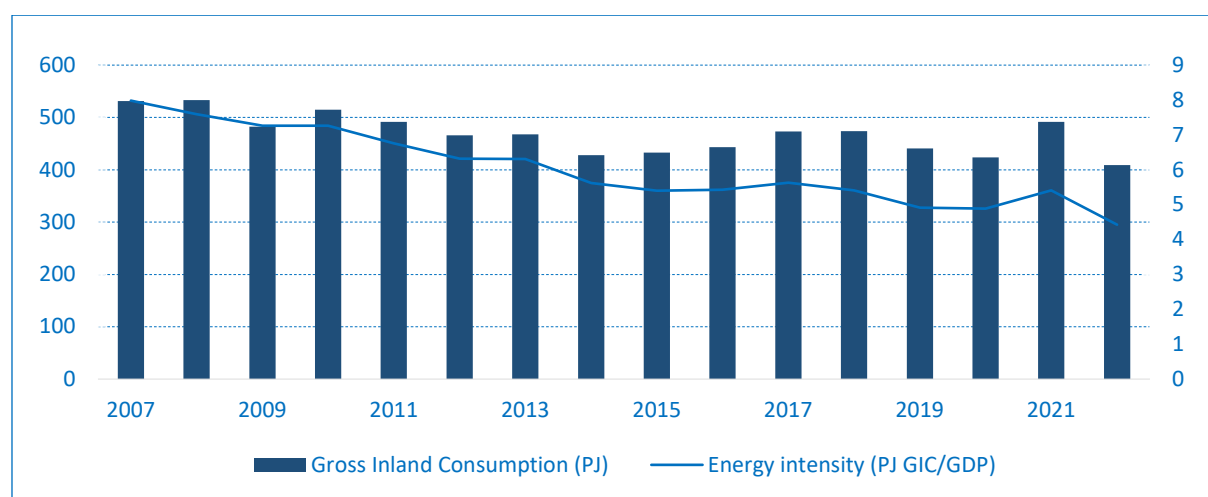
Figure 3.3: The trend of energy intensity (right y axis) in the period 2007 – 2022 (estimated by the revised statistical approach NACRev.2)
